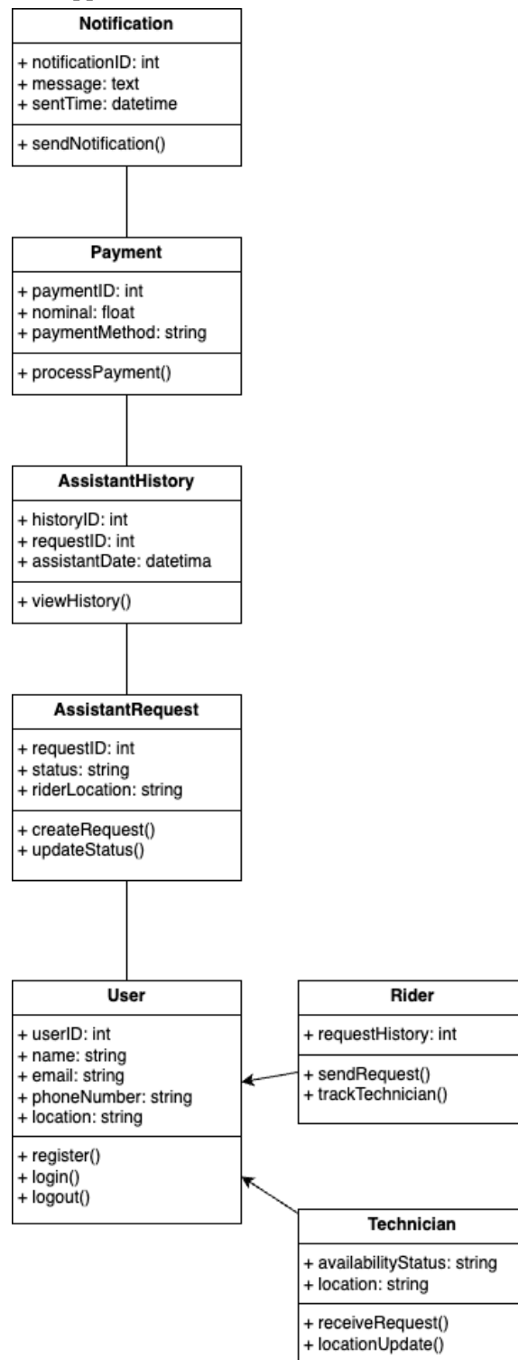
Fig. 2. Class Diagram
