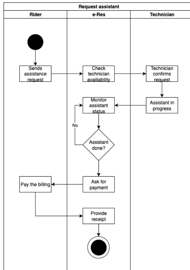
Fig. 4. Activity Diagram
