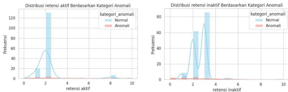
Figure 10. Distribution of Retention Periods by Anomaly Category
