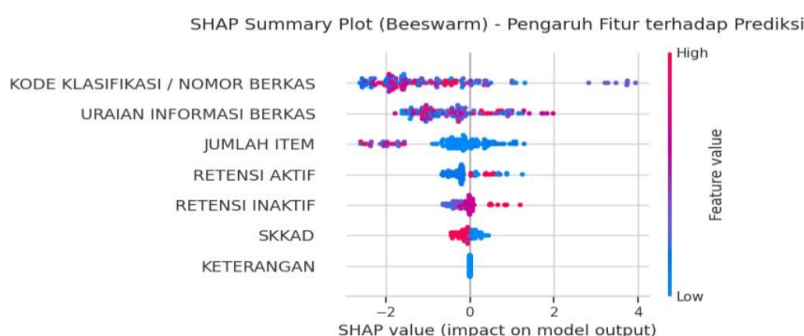
Figure 5. SHAP Summary Plot of Influential Features in Archival Classification
